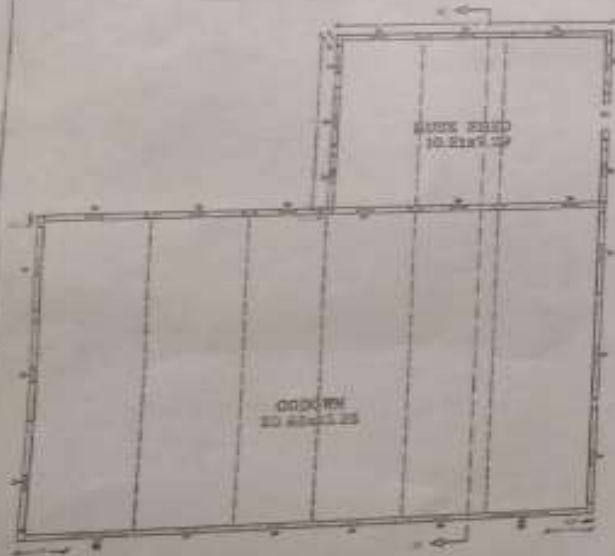
GODOWN & HUSK SHED PLAN
